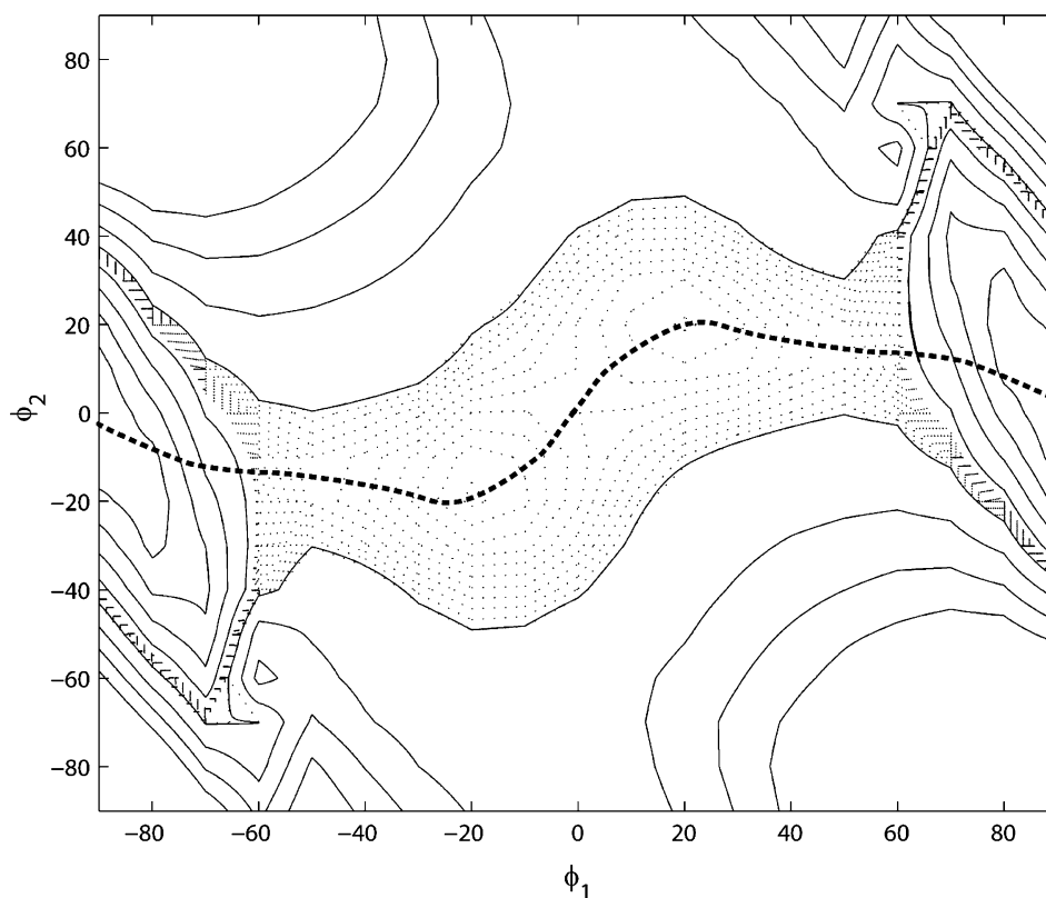
Figure 11. Contour plot of the excited-state potential energy surface of TO as a function of \phi_1 and \phi_2 , obtained from the hybrid method. The dotted contours are from 2.60 to 2.65 eV in steps of 0.005 eV. The solid contours begin at 2.65 eV with increments of 0.1 eV. The bold dotted line shows the lowest energy path for the twisting motion. This path has a local maximum at (\phi_1, \phi_2) = (0^\circ, 0^\circ) . Shallow local minima at about \phi_1 = \pm 20^\circ are separated from deep minima at \phi_1 = \pm 90^\circ by a barrier at \pm 60^\circ (compare to Figure 10).
