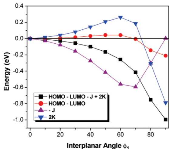
Figure 9. Individual contributions of energy terms given in eq 1 to the excited-state energy of TO as a function of the interplanar angle \phi_1 , holding \phi_2 fixed at 0^\circ .
