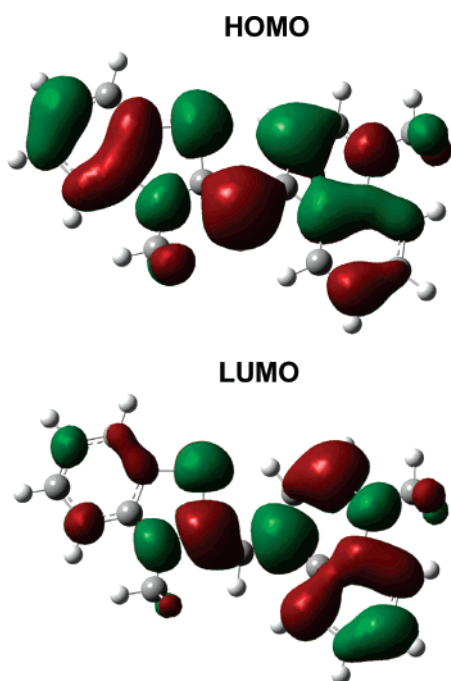
Figure 4. HOMO and LUMO of TO obtained from SAM1 computations on the ground-state structure. The molecules are drawn oriented as shown in Chart 1.
