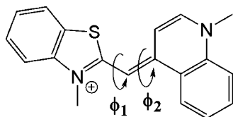
Figure 6. Definition of interplanar angles, \phi_1 and \phi_2 , used to describe twisting of TO.
