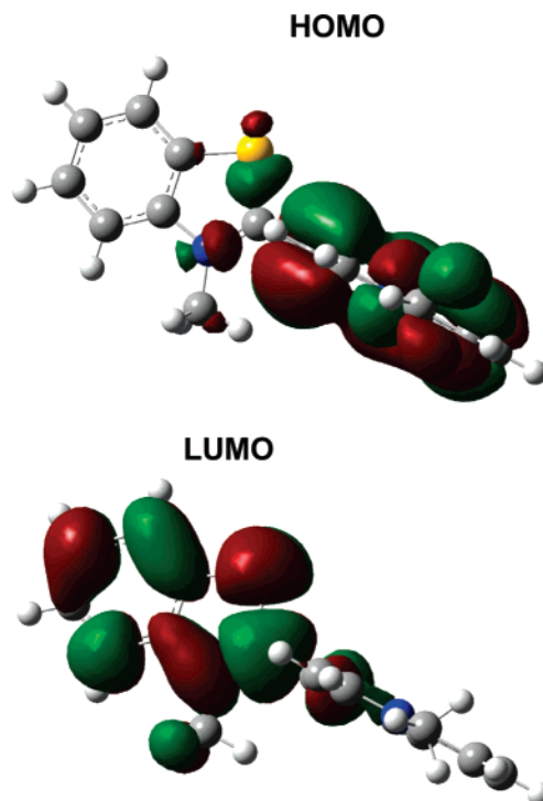
Figure 8. HOMO and LUMO of TO obtained from SAM1 computations on the 90^\circ twisted structure. The molecules are drawn oriented as shown in Chart 1.
