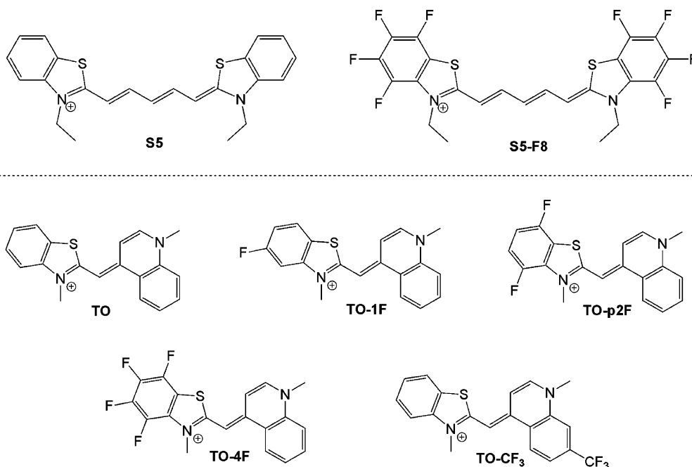
Chart 1. Fluorinated and Nonfluorinated Cyanine Dyes a
