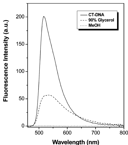
Figure 5. Fluorescence spectra recorded for 1.0 \mu\text{M} TO-p2F in methanol (dotted), 90% glycerol–water (dashed), and double-stranded calf thymus (CT) DNA (solid). Spectra were corrected for differences in absorbance at the excitation wavelength (450 nm).
