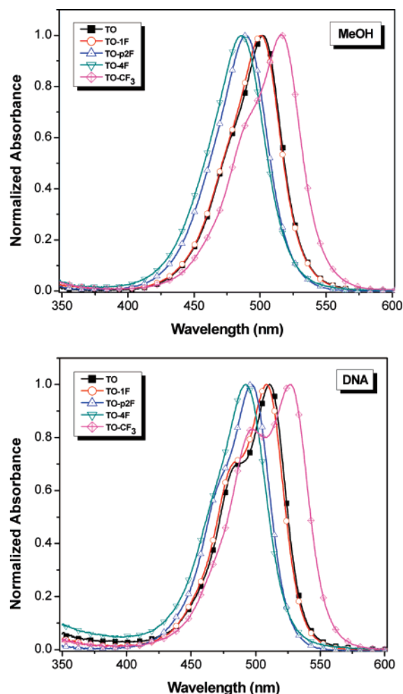
Figure 1. UV-vis absorption spectra of TO and fluorinated analogues determined in methanol (top) and in the presence of double-stranded DNA (bottom). Each spectrum was normalized at its wavelength of maximum absorbance.
