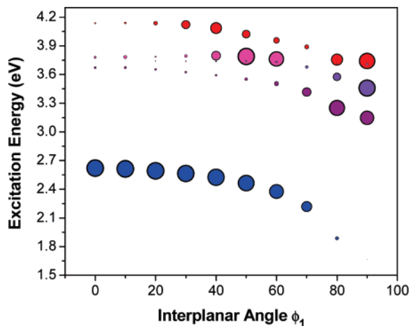
Figure 7. Singlet excitation energies of TO as a function of the interplanar angle \phi_1 , holding \phi_2 fixed at 0^\circ (angles defined in Figure 6). The radius of the circles is proportional to the predicted absorption intensity. The excitation energies for the S0–S1 transition are shown in blue, while energies for transitions to higher states are shown in purple (S0–S2), violet (S0–S3), magenta (S0–S4), and red (S0–S5).
