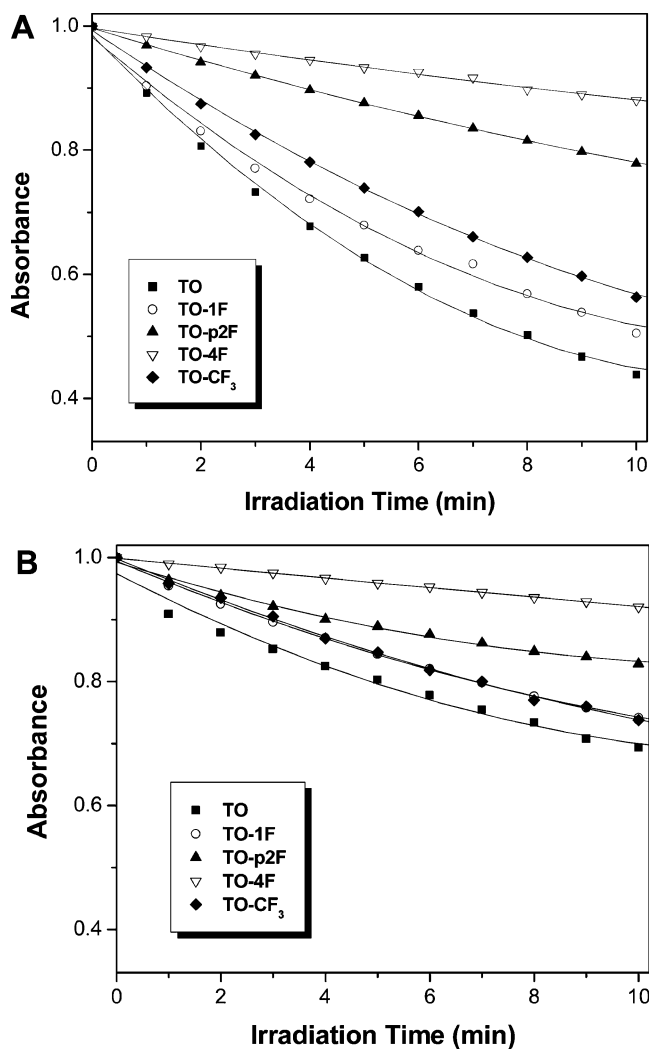
Figure 13. Absorbance of 5.0 \mu\text{M} dye solutions irradiated with visible light for 1 min time intervals in either aqueous buffer (A) or 100 \mu\text{M} base pairs CT-DNA (B).
